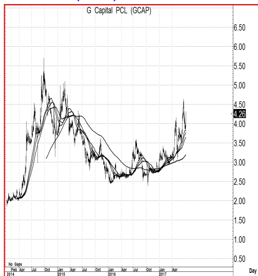
Price Chart...(GCAP)
